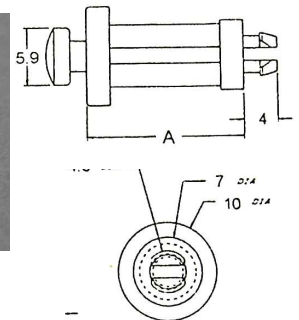
PYP PCB Hole 4.0mm
